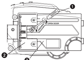
Battery Installation
